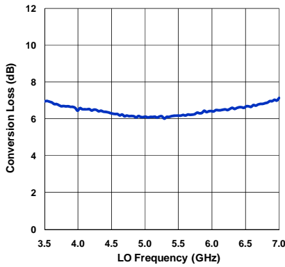
Conversion Loss
