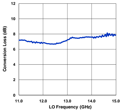
Conversion Loss
