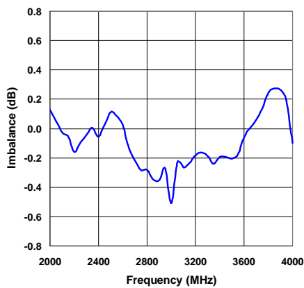
Amplitude Imbalance
