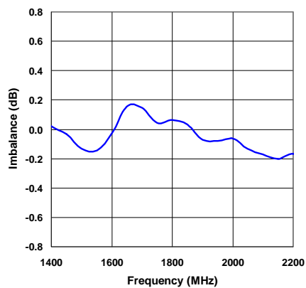
Amplitude Imbalance
