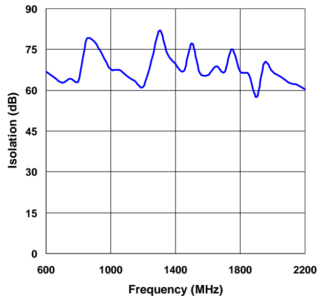
LO-RF Isolation
