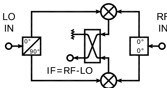
BLOCK DIAGRAM ( IF=RF-LO CONFIGURATION)
